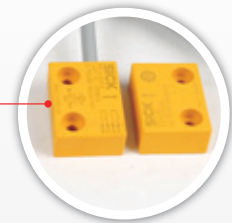
\\ Door Safety Switch The laser welding machine would stop immediately when the door is open.
